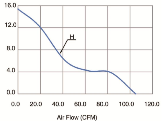
■ Performance Curves
