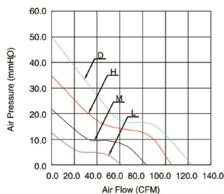
■ Performance Curves
