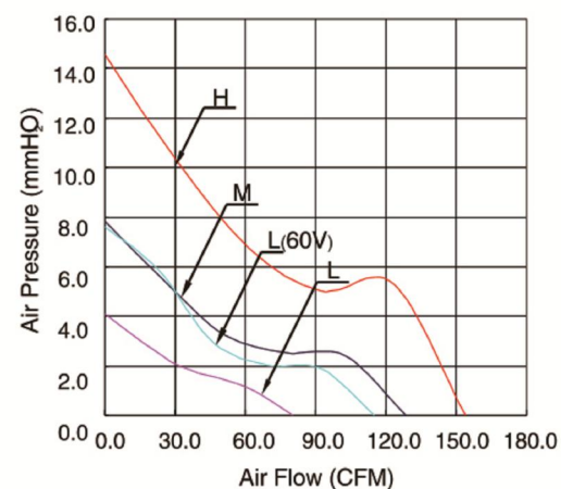
■ Performance Curves
