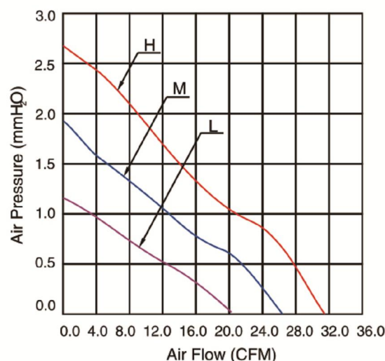
■ Performance Curves
