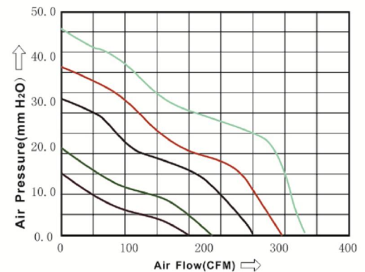
■ Performance Curves
